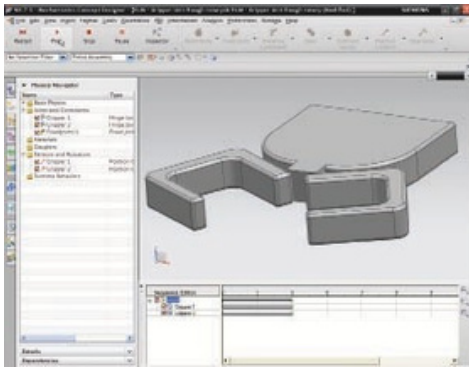
Mechatronics Concept Designer facilitates re-use of objects embedded with mechatronics knowledge. This gripper includes correct kinematic motion information.
